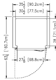
Plan - R/ARI132HUT
