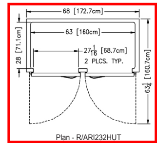
Plan - R/ARI232HUT
