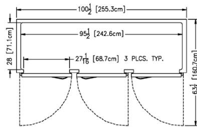
Plan - R/ARI332HUT
