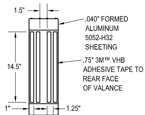
DECORATIVE REVEAL FRONT VIEW SCALE 1" = 1'
