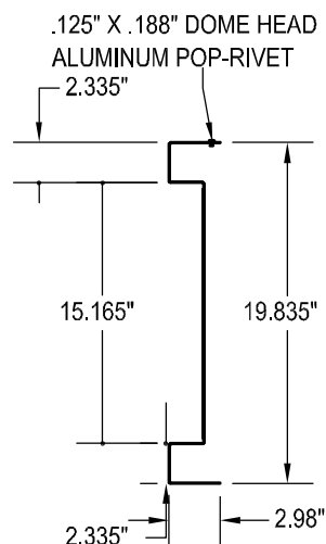
SIDE VIEW SCALE 1" = 1'
