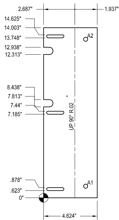
PART 2 FLAT PATTERN SCALE 1/4" = 1"
