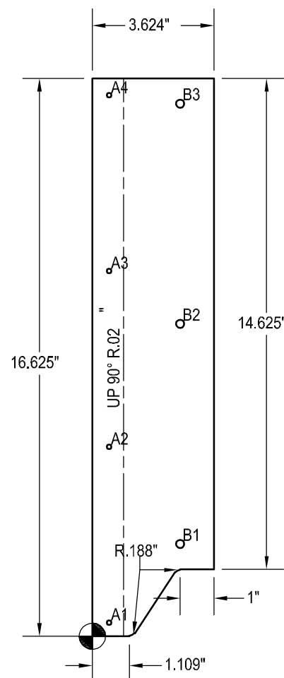
PART 1 FLAT PATTERN SCALE 1/4" = 1"
