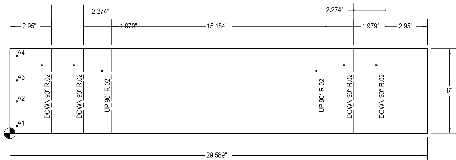
DECORATIVE REVEAL FLAT PATTERN SCALE 1/4" = 1"
